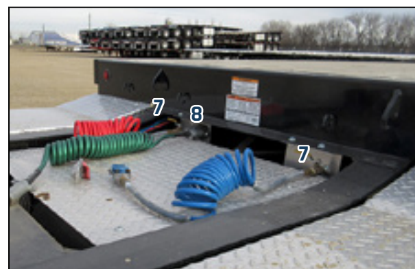
Figure 11 – Branchements (type)
