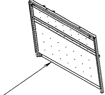
10AH0466W FRONT WALL ASSY, AHV PUP, 82", WHITE, SS REV B
